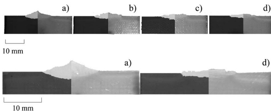
Figure 7. LM pictures on selected DEN-T specimens at the same ligament length ( L = 13 mm) for (a) EPBC, (b) EPBC-BA-1, (c) EPBC-BA-2.5, (d) EPBC-BA-5. Note that the composed picture show the same plastic zone in contrasted (image processing) and original forms (left and right sides, respectively).
