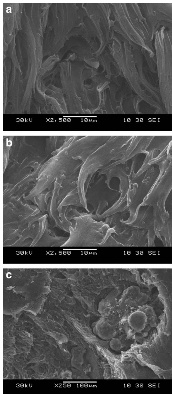
Figure 8. (a) fracture surface of the DEN-T specimen of EPBC-BA-1, magnification: 2500 \times ; (b) fracture surface of the DEN-T specimen of EPBC-BA-5, magnification: 2500 \times ; (c) five fracture surface of the DEN-T specimen of EPBC-BA-5, magnification: 250 \times .
