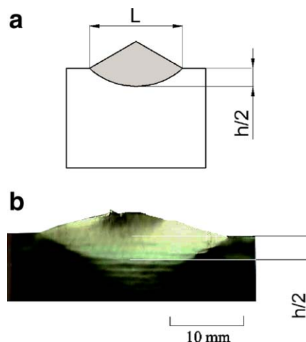
Figure 5. Determination of the \beta shape factor by measuring the half height of plastic deformation zone: (a) plastic deformation zone and measuring of h/2 schematically, (b) stripes under the plastic zone on a broken DEN-T specimen. [Color figure can be viewed in the online issue, which is available at wileyonlinelibrary.com .]
