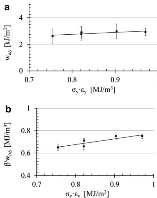
Figure 6. Yielding-related specific essential ( w_{e,y} ; a) and non-essential work of fracture terms ( \beta' w_{p,y} ; b) as a function of \sigma_y \epsilon_y .
