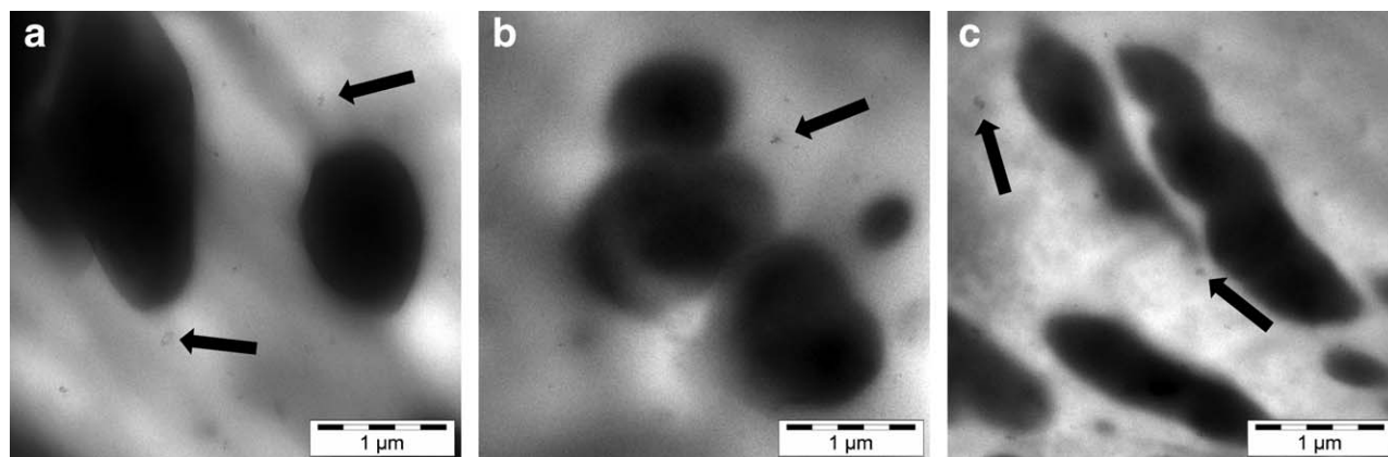
Figure 1. TEM micrographs of the EPBC-BA nanocomposites at different BA contents: (a) 1.0 wt %; (b) 2.5 wt %; (c) 5.0 wt %.
