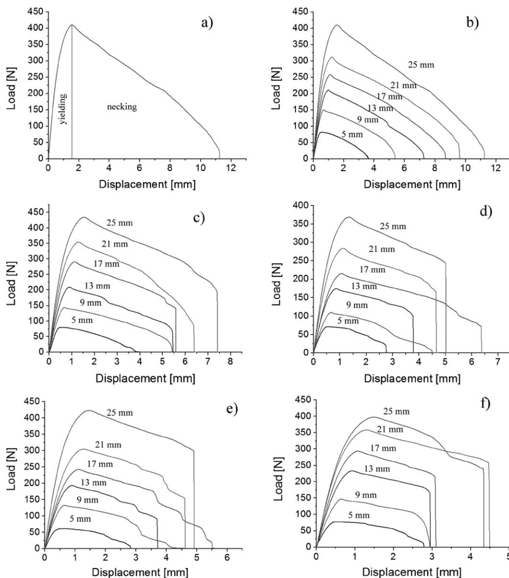
Figure 3. Curve partitioning in principle and selected F - x curves of the EPBC-BA nanocomposites, (a) splitting between yielding and necking zones, (b) EPBC, (c) EPBC-BA-0.5, (d) EPBC-BA-1, (e) EPBC-BA-2.5, (f) EPBC-BA-5. The numbers above the curves refers to the ligament lengths. Note that with increasing nanoparticle contents the DEN-T specimens' broke in an unstable manner in the necking/tearing stage. This means that the nanoparticles hampered the plastic work dissipation which is well reflected by the EWF results (Table II).
