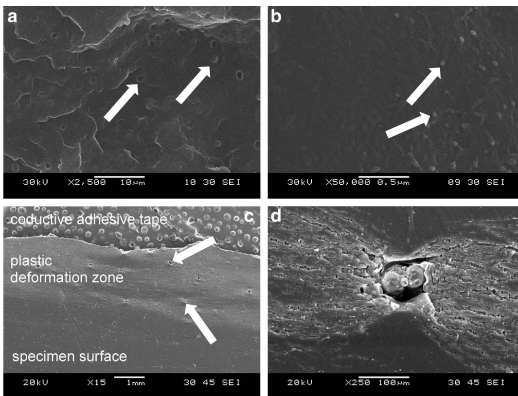
Figure 2. SEM micrographs taken from EPBC-BA nanocomposites: (a) cryo-fractured EPBC-BA-1, magnification: 2500 \times ; (b) cryo-fractured EPBC-BA-1, magnification: 50,000 \times ; (c) surface view of fractured DEN-T specimen from the plastic zone of EPBC-BA-5, magnification: 15 \times ; (d) surface view of fractured DEN-T specimen from the plastic zone of EPBC-BA-5, magnification: 250 \times .
